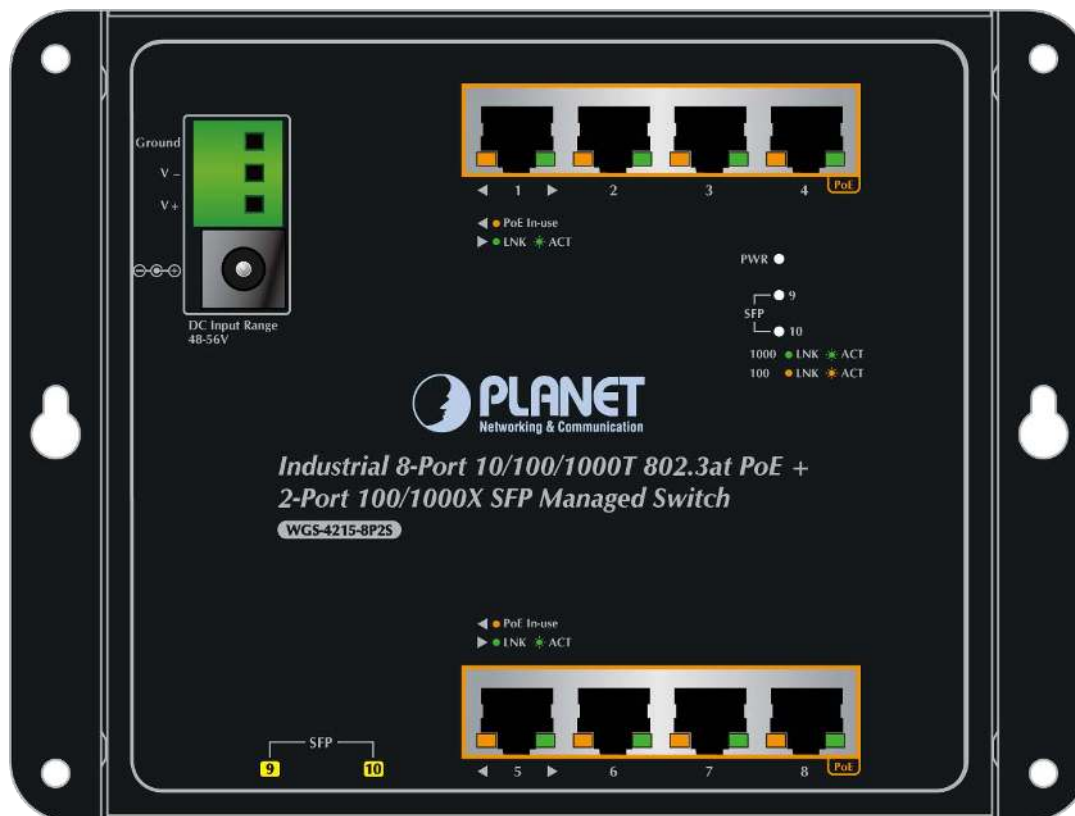
Figure 2-1-2d WGS-4215-8P2S LED Panel
