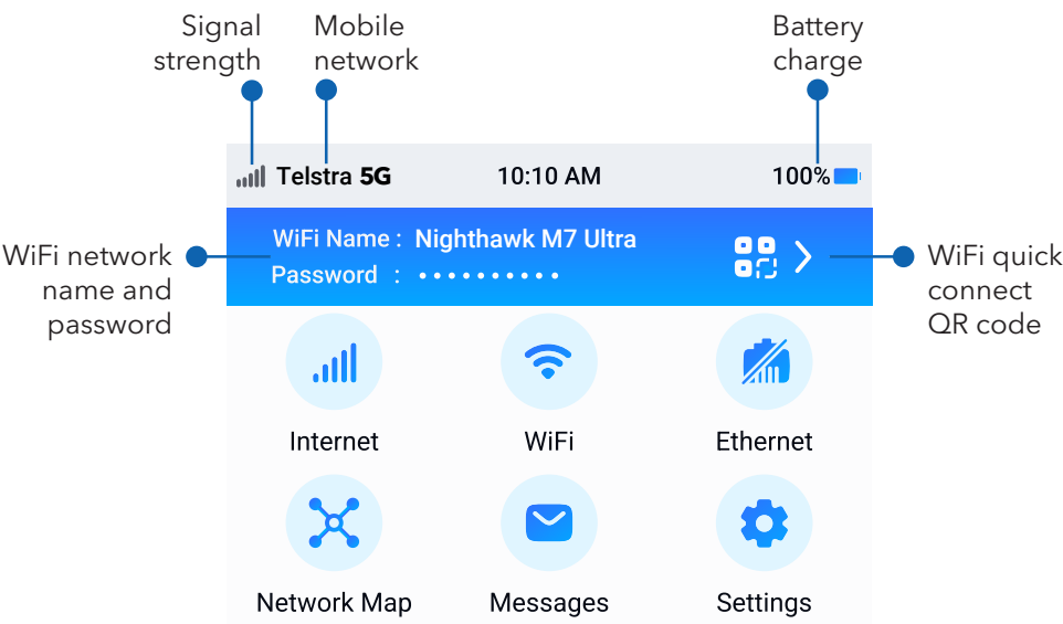
Figure 8. Home screen
